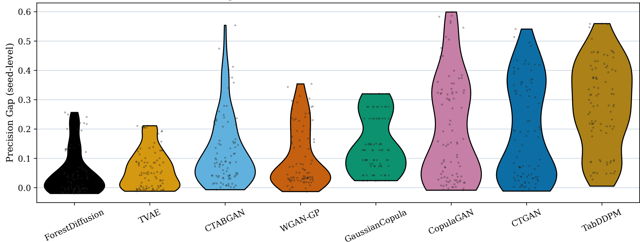
Precision Gap — seed-level distribution (n = 10 seeds × datasets)
